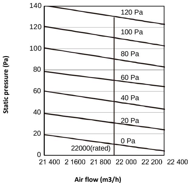
Figure 3-3.11: 18-30HP units fan performance
