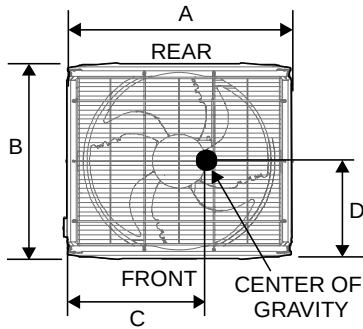
Figure 3-2.9: 18-30HP Center of gravity
