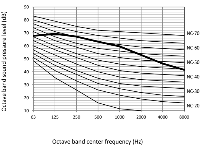
Figure 2-10.13: 30HP octave band level
