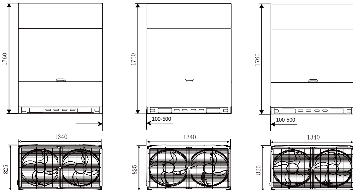
Figure 2-2.10: 78/80/82/84/86/88/90HP dimensions (unit: mm)
