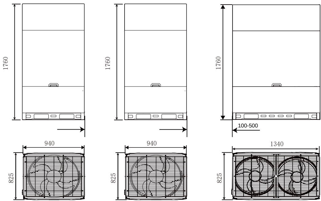
Figure 2-2.8: 62HP dimensions (unit: mm)
