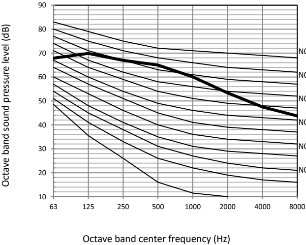
Figure 2-10.12: 28HP octave band level
