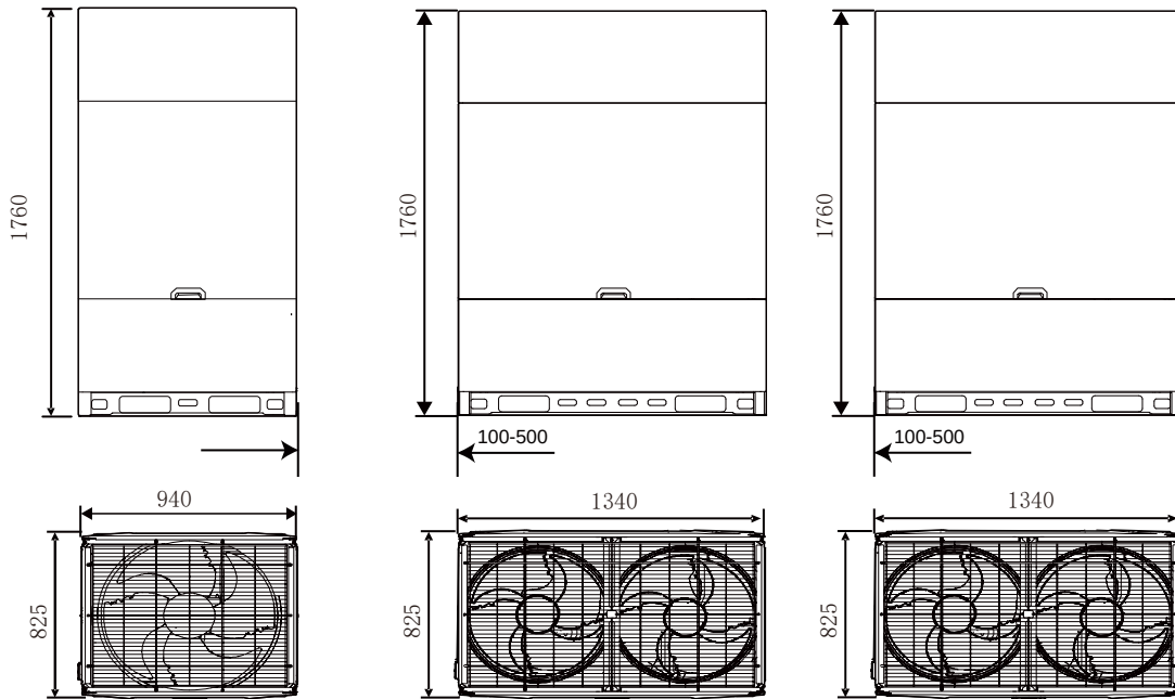
Figure 2-2.9: 64/66/68/70/72/74/76HP dimensions (unit: mm)
