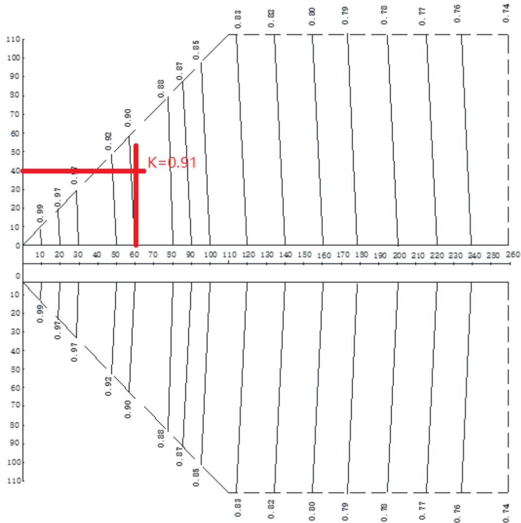
Figure 1-6.3: SUPER YC rate of change in cooling capacity
