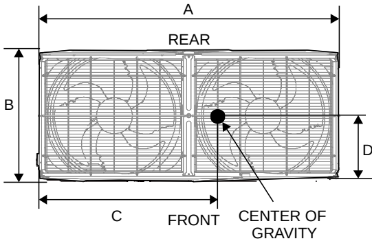
Figure 3-2.9: 18-30HP Center of gravity
