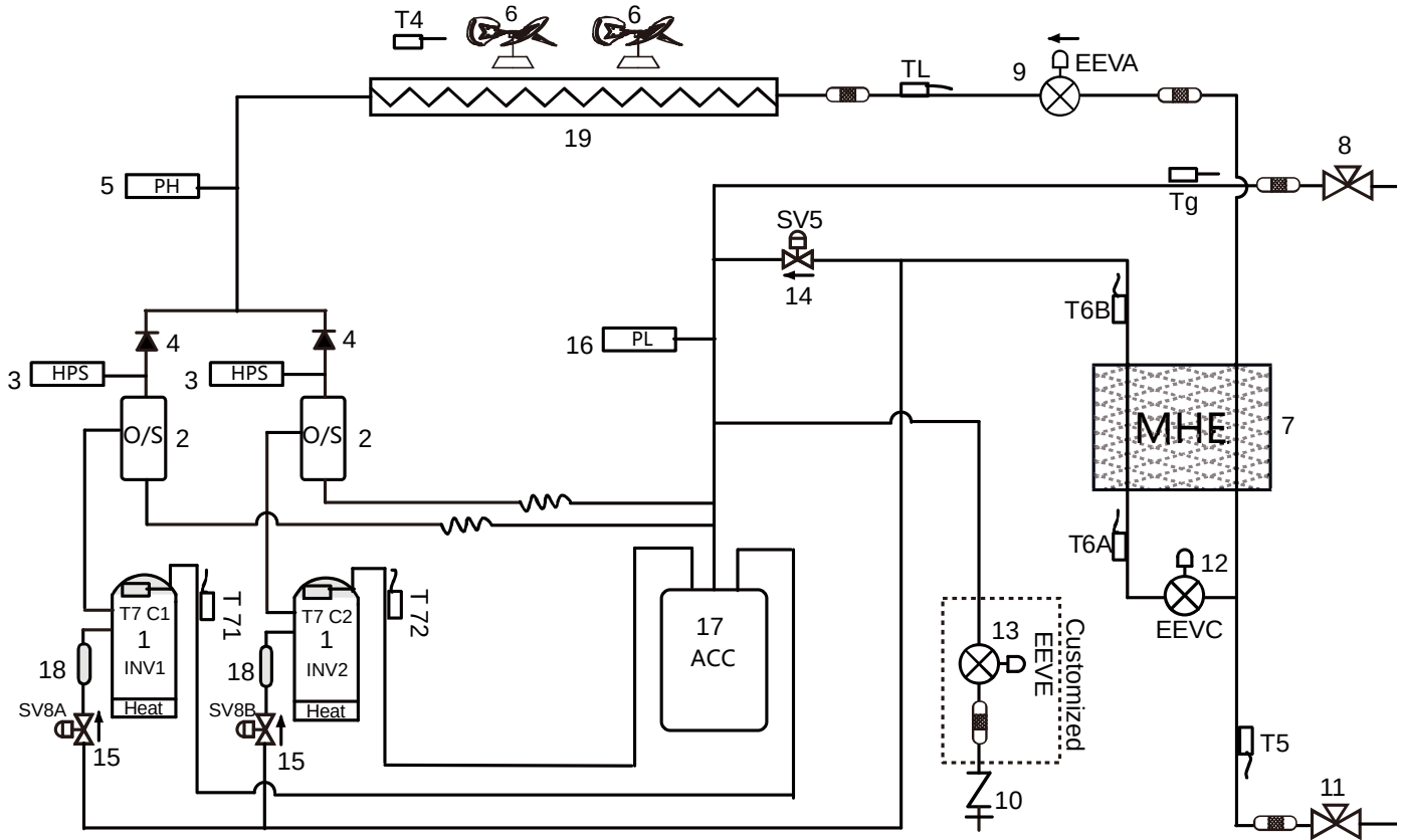
Figure 2-4.3: 18-24HP piping diagram
