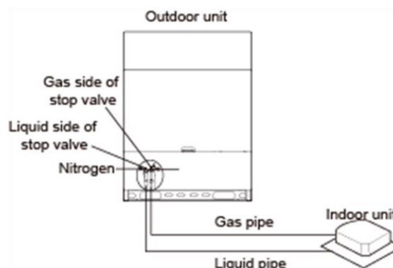
Figure 3-5.14: Gastightness test
