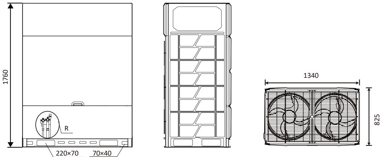
Figure 2-2.2: 18/20/22/24/26/28/30HP dimensions (unit: mm)
