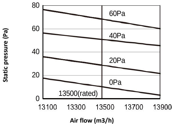
Figure 3-3.9: 8-12HP units fan performance
