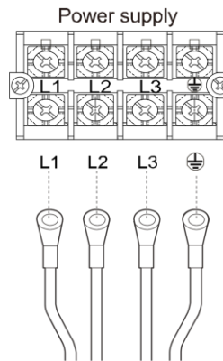
Figure 3-9.4: Outdoor unit power supply terminals
