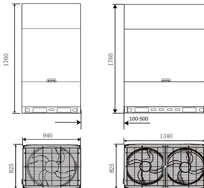
Figure 2-2.6: 34/36/38/40/42/44/46HP dimensions (unit: mm)
