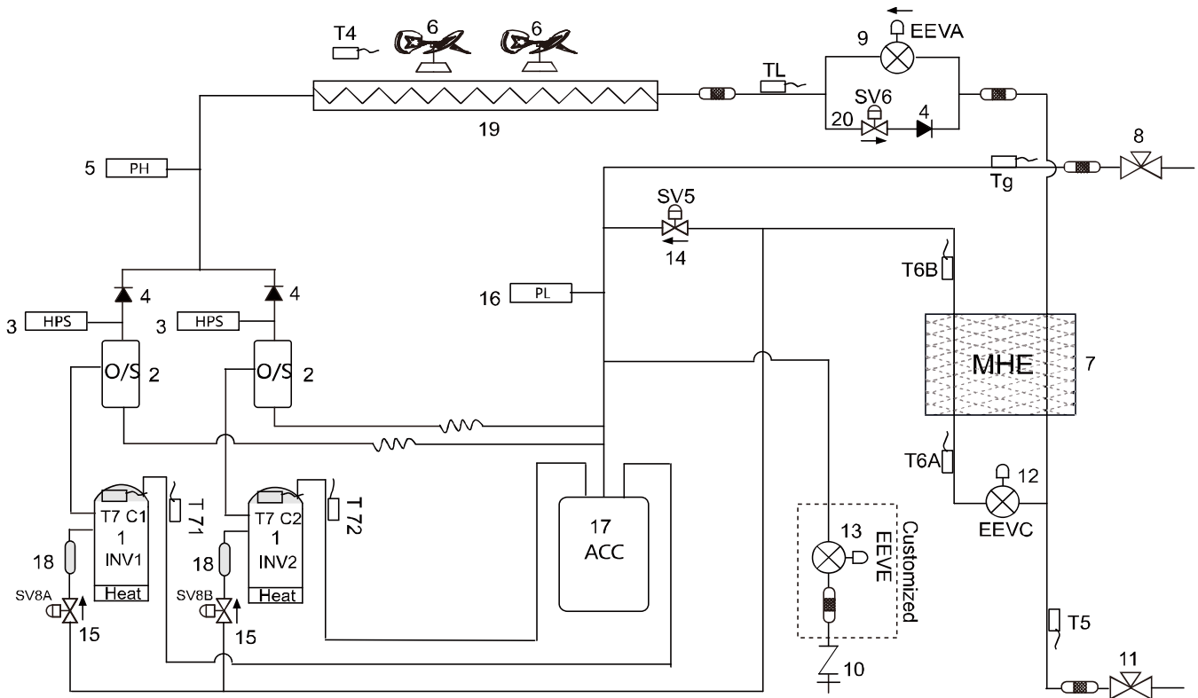
Figure 2-4.3: 26-30HP piping diagram
