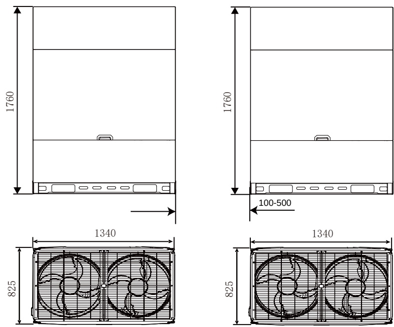
Figure 2-2.7: 48/50/52/54/56/58/60HP dimensions (unit: mm)
