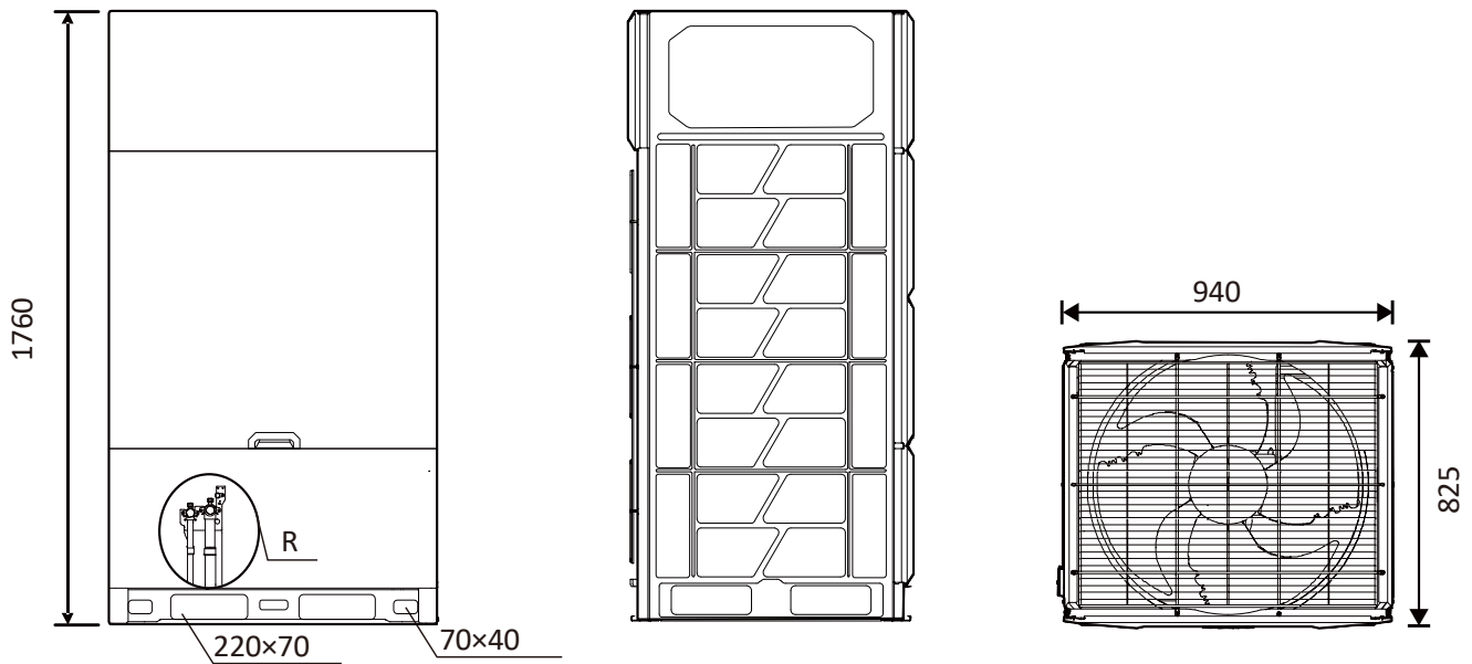
Figure 2-2.1: 8/10/12/14/16HP dimensions (unit: mm)
